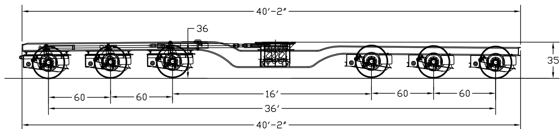
FRONT GROUP SELF STEER FROM BOLSTER
