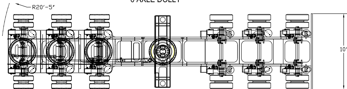
6 AXLE DOLLY
