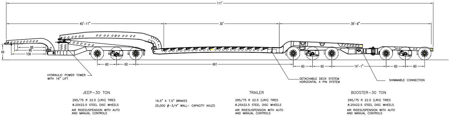
13 AXLE 85 TON HEAVY HAUL TRAILER SYSTEM
