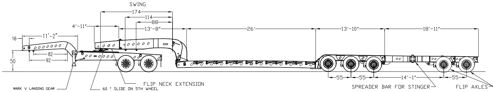
65 TON HYDRAULIC GOOSENECK MODULAR SYSTEM WITH OPTIONAL FLIP NECK AND STINGER AND JEEP
